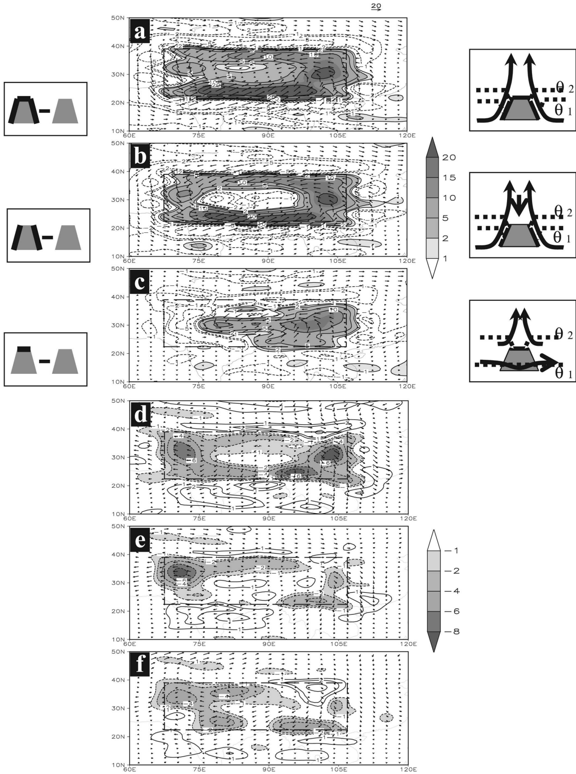
FIG. 4. Distributions of difference wind (vectors; m s^{-1} ) and vertical velocity ( -\omega ; shading; 10^{-2} Pa s^{-1} ) at the \sigma = 0.991 surface from the perpetual July experiments (a) ALLSH-NOSH, (b) SLPSH-NOSH, and (c) TOPSH-NOSH and from the perpetual January experiments (d) ALLSH-NOSH, (e) SLPSH-NOSH, and (f) TOPSH-NOSH. The rectangle in (a)–(f) indicates the mountain domain. Left panels indicate the experiment designs, and right panels indicate mechanism interpretations. See text for details.
